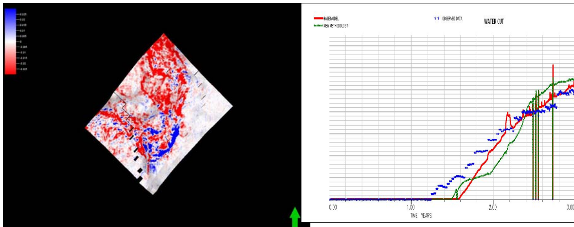
Figure 2. The results of the flow simulations: water cut in the Producer. The comparison of the results of simulations with full field model (red), new methodology model (green), and observed data (blue).
