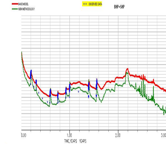
Figure 4. The results of the flow simulations: static and flow bottom hole pressures in the Producer. The comparison of the results of simulations with full field model (red), new methodology model (green), and observed data (blue).
